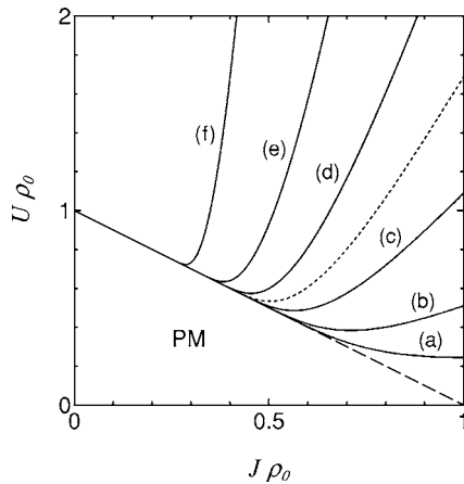
FIG. 3. Contour lines for various ratios T_{AF}/T_c in the J - U plane. The solid curves (a)–(f) are the contour lines for \alpha=2, 3, 5, 10, 20 , and 100 , respectively, where \alpha \equiv (T_{AF}\rho_0/n)/(T_c/W_c) = T_{AF}/T_c \times W_c\rho_0/n . The dotted curve is that of \alpha=7 , which corresponds to the experimental result of \text{UPd}_2\text{Al}_3 . The dashed curve shows the phase boundary between the antiferromagnetic and paramagnetic (PM) phases at T=0 .
