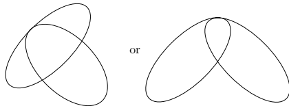
FIGURE 8.1. The configurations of smooth conics for qq
