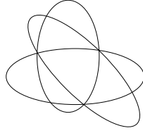
FIGURE 8.2. The configuration of smooth conics for \mathbf{tq1}
