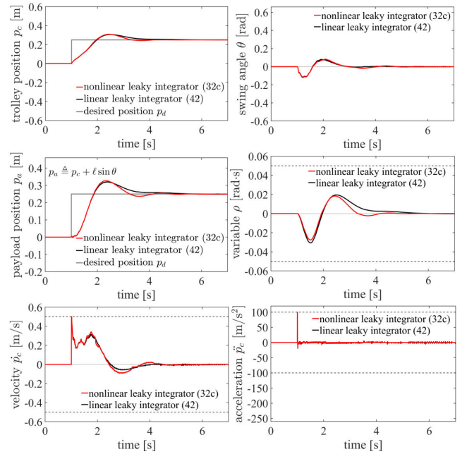
FIGURE 7. Experiment IV: effects of the nonlinear leaky integral controller.
