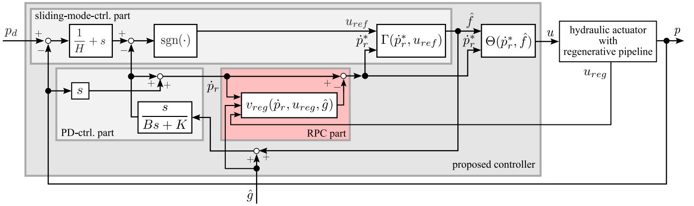
Fig. 5. Block diagram of the proposed controller with the regenerative-pipeline compensation (RPC). The opening ratio u_{reg} of the regenerative pipeline is determined by the built-in controller of the actuator and is assumed to be readable from the proposed controller. The set-valued functions \Gamma and \Theta are determined according to the structure of the hydraulic circuit.
