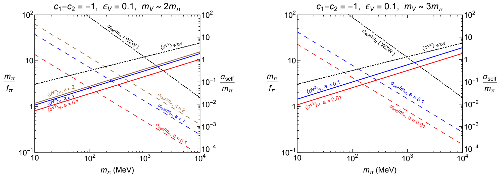
FIG. 2: Contours of relic density ( \Omega h^2 \approx 0.119 ) for m_\pi and m_\pi/f_\pi and self-scattering cross section in \text{cm}^2/\text{g} as a function of m_\pi . The case without and without vector mesons are shown in black lines and colored lines respectively. Vector meson masses are taken near the resonance with m_V \approx 2m_\pi ( m_V \approx 3m_\pi ) on left(right) plots. In both plots, c_1 - c_2 = -1 and \epsilon_V = 0.1 are taken.
