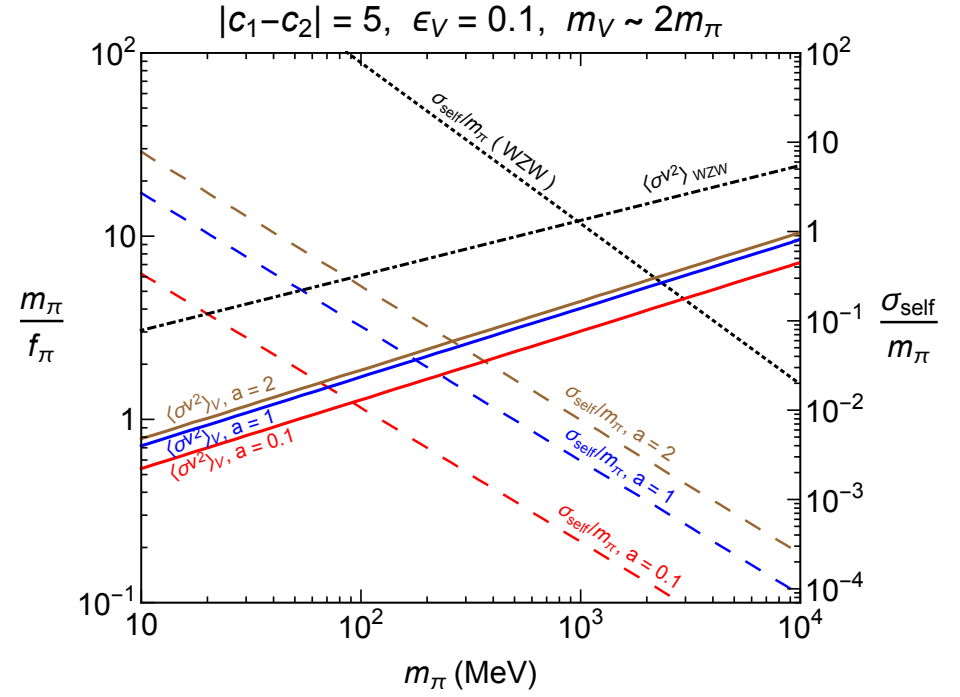
FIG. 3: Similar contours of relic density for m_\pi and m_\pi/f_\pi and self-scattering cross section per DM mass as in Fig. 2. Vector meson masses are taken near the resonance with m_V \approx 2m_\pi , and |c_1 - c_2| = 2, 5 is chosen.
