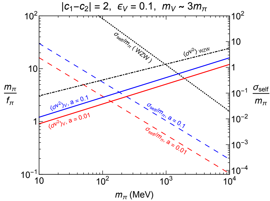
FIG. 4: Similar contours of relic density for m_\pi and m_\pi/f_\pi and self-scattering cross section per DM mass as in Fig. 2. Vector meson masses are taken near the resonance with m_V \approx 3m_\pi , and |c_1 - c_2| = 2, 5 is chosen.
