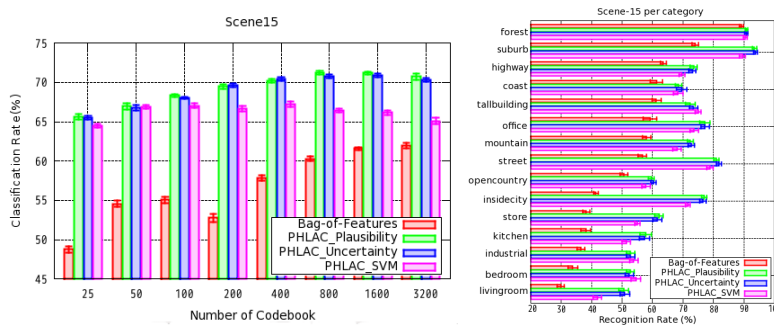
Fig. 6. Recognition Rates of Scene15: per codebook size (left) and per category when codebook size is 200(right)
